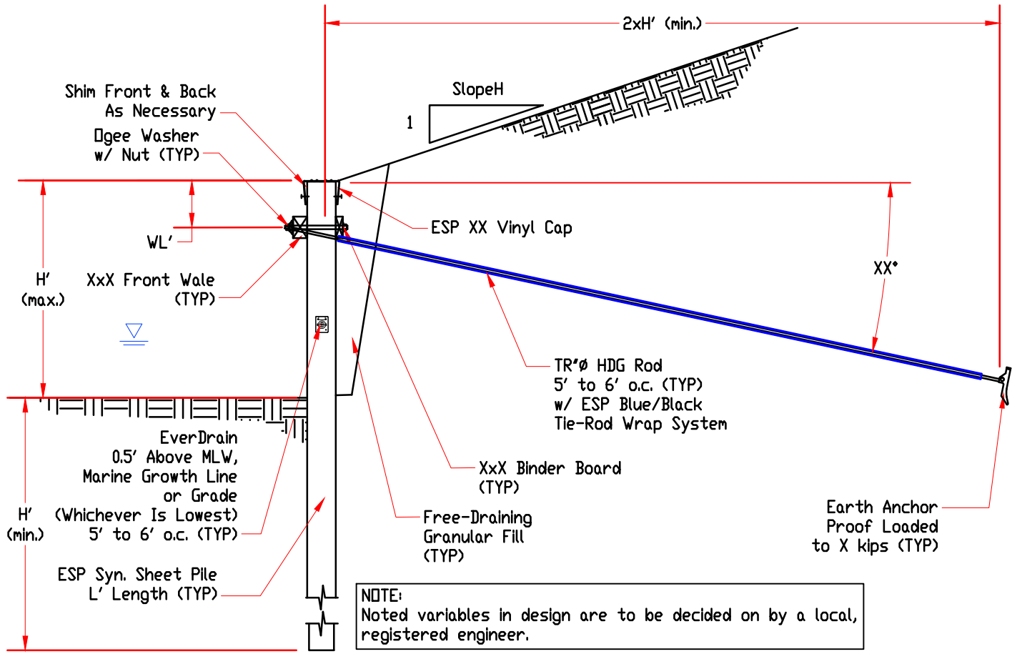
Typical Section
