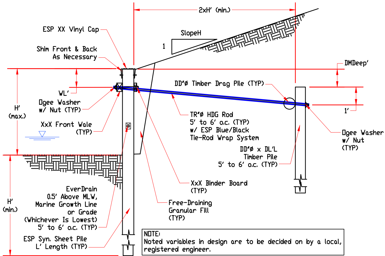
Typical Section
