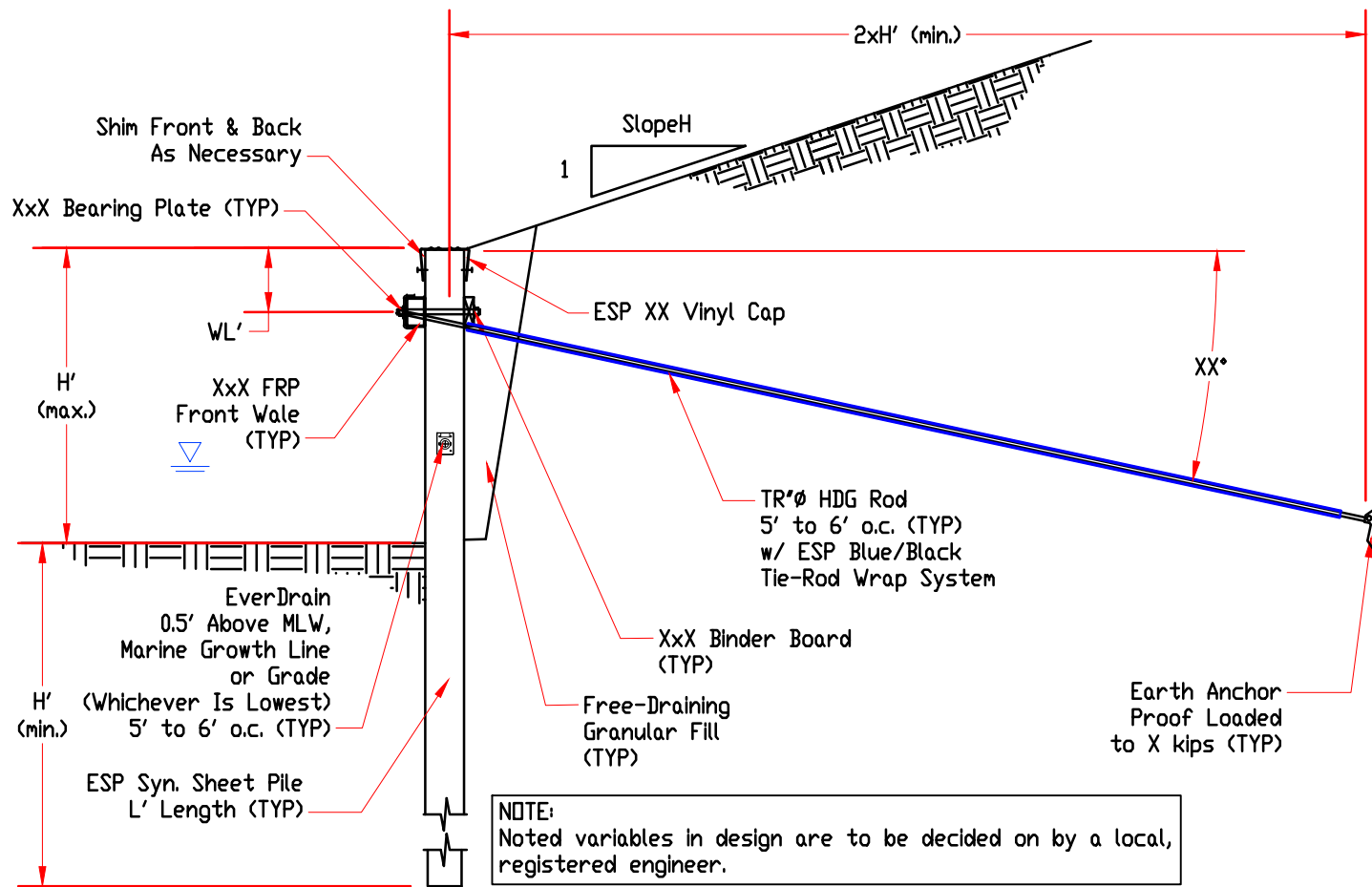
Typical Section
